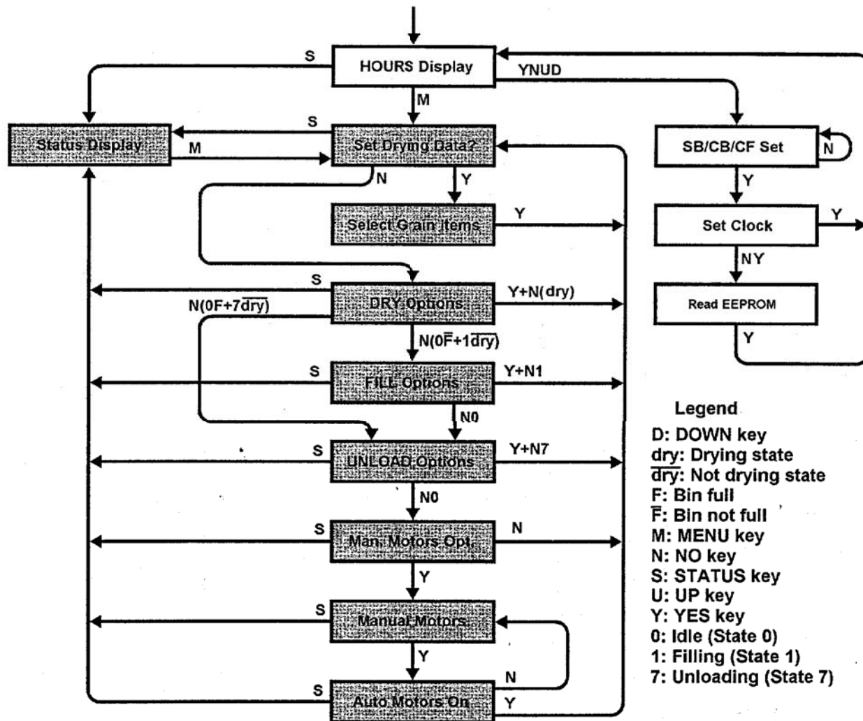
Figure 5A - Path to the initialization routines.
