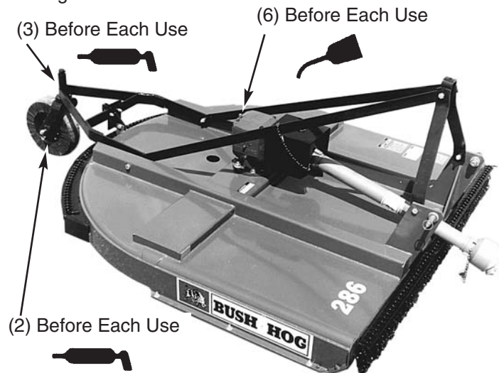
Figure 4-1 Lubrication
