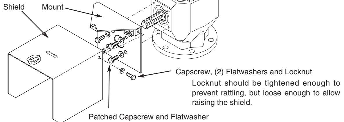
Figure 5-6 Clutch Shield
